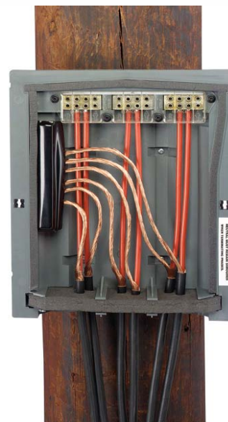
Type 1a ABC service box mounted to pole
